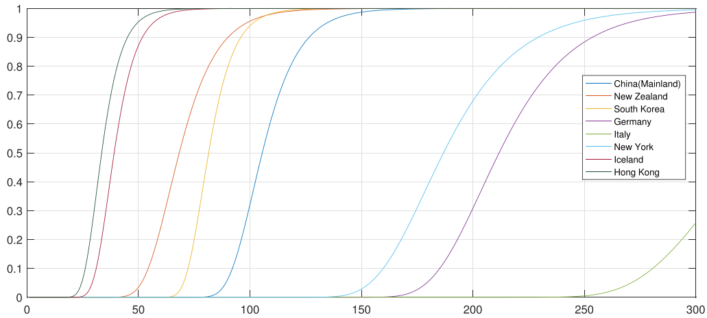
Fig. 10. Conditional elimination probability \mathbb{P}(\tilde{T} \leq t | \tilde{S} \leq t) for China (Mainland), New Zealand, South Korea, Germany, Italy, New York, Iceland and Hong Kong under the associated calibration parameters (\hat{\alpha}, \hat{\beta}, \hat{\delta}, \hat{\varrho}, \hat{\ell}) for these regions and countries suggested in Table 3.
